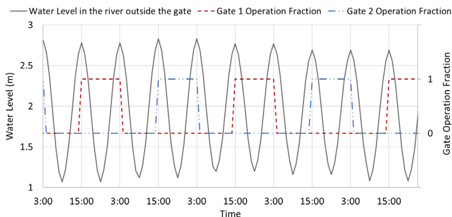
FIGURE 6 The cyclicity of water level in the river outside the gate and operation of the gates (1 = open, 0 = closed) for the scenario with 'successive' gate operation
